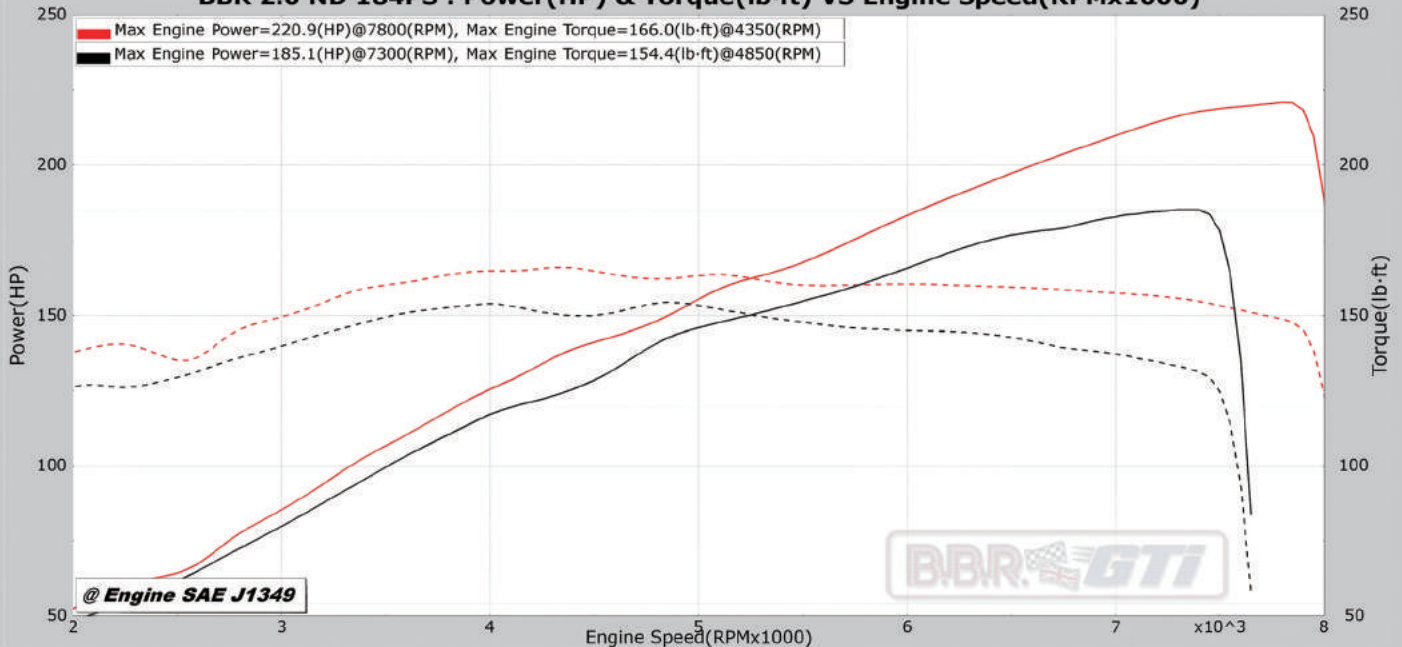
BBR 2.0 ND 184PS : Power(HP) & Torque(lb-ft) VS Engine Speed(RPMx1000)
