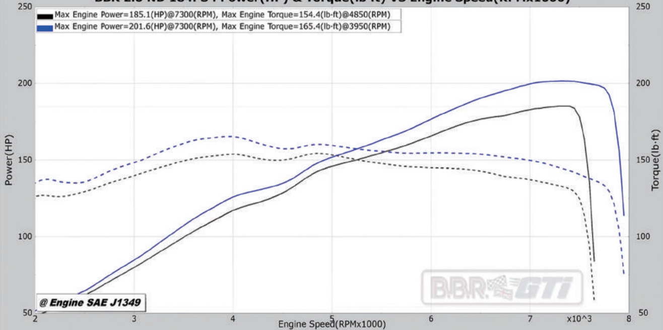
BBR 2.0 ND 184PS : Power(HP) & Torque(lb-ft) VS Engine Speed(RPMx1000)
